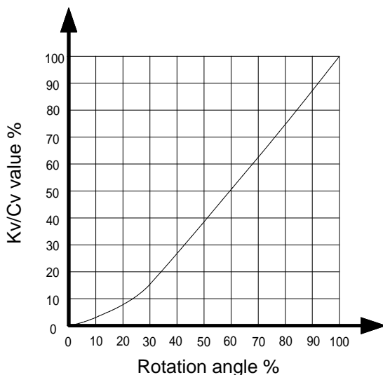
Fig. 5: Natural characteristic
