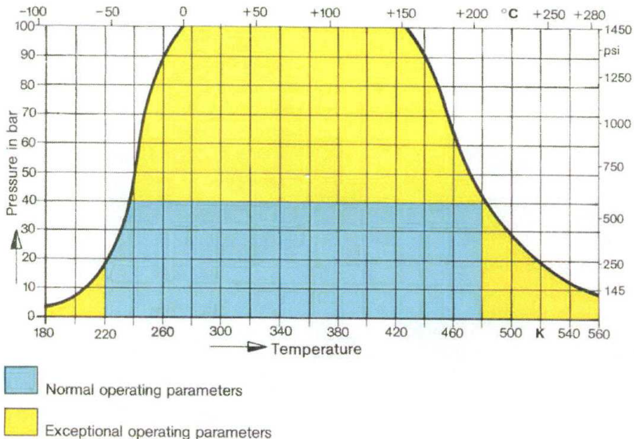
Figure 2, Sleeved Plug Valve Pressure-Temperature Chart
